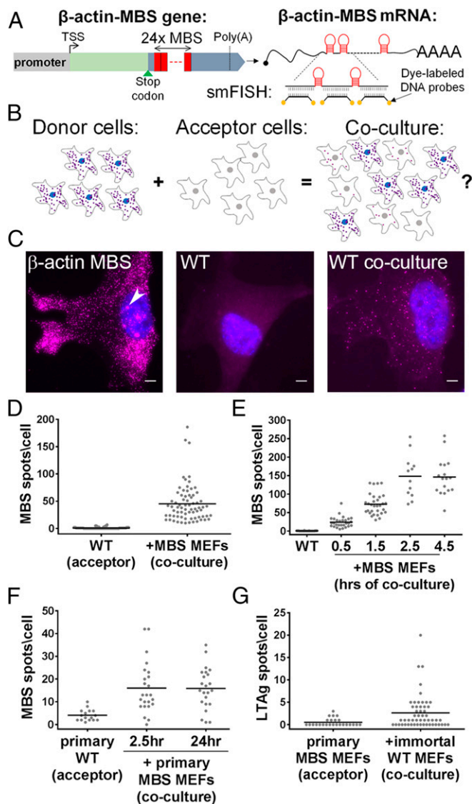
Fig. 1. Detection of \beta -actin–MBS mRNA transfer by smFISH. (A) A schematic depicting the \beta -actin–MBS gene (Left) and resulting mRNA (Right). mRNA detection was accomplished using smFISH with fluorescence-labeled DNA probes against the MBS sequence (aka “MBS probes”). Poly(A), polyadenylation site; TSS, transcription start site. (B) A schematic illustrating the basic experimental set-up. Donor cells (Left) that express a unique mRNA (e.g., \beta -actin–MBS; shown as small purple dots) were cocultured with naive acceptor cells (Middle) that lack this mRNA. If mRNAs undergo transfer from donor to acceptor cells, coculture yields labeling of the acceptor cells (Right). Each cell type was also cultured separately to assess mRNA-expression levels in donor cells or background staining in acceptor cells. (C) smFISH images of an immortalized donor MBS MEF, immortalized acceptor WT MEF, and acceptor WT MEF in coculture. Labels: blue, DAPI staining of the nucleus; magenta, Cy3-tagged MBS probes. The arrowhead indicates a transcription site. (Scale bars: 5 \mu m.) (D) Distribution of the number of \beta -actin–MBS mRNA spots observed in immortalized WT MEFs (expressing low levels of GFP) cultured alone or cocultured with donor MBS MEFs for 24 h. Each dot in D–G represents the score of the number of mRNAs detected in a single cell as obtained by smFISH. The horizontal bars in D–G indicate mean number of spots per acceptor cell. (E) Distribution of the number of \beta -actin–MBS mRNA spots in WT MEFs as a function of time after coculture with donor MBS MEFs. (F) Distribution of the number of \beta -actin–MBS mRNA spots in primary WT MEFs cultured alone or cocultured for 2.5 or 24 h with primary donor MBS MEFs. (G) Distribution of the number of LTag mRNA spots in primary MBS MEFs cocultured with LTag-immortalized donor WT MEFs for 24 h. See Dataset S1 for data on the number of cells scored, mean, SEM, and P values for each experiment.
